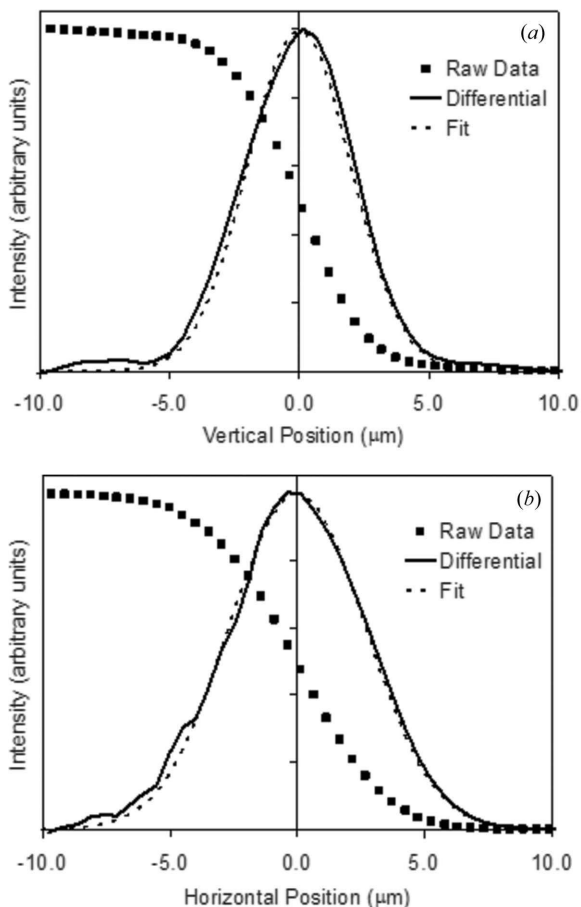
Figure 6 Profiles of the mini-beam defined by the 5 \mu\text{m} aperture in the vertical ( a ) and horizontal ( b ) directions. Profiles were recorded at the sample position using a knife-edge scan as described in the text. The raw knife-edge scans were differentiated, providing the beam profile (solid line). An error function was fit to the raw data (not shown). The best-fit Gaussian is derived from the derivative of the error function (dashed line).
