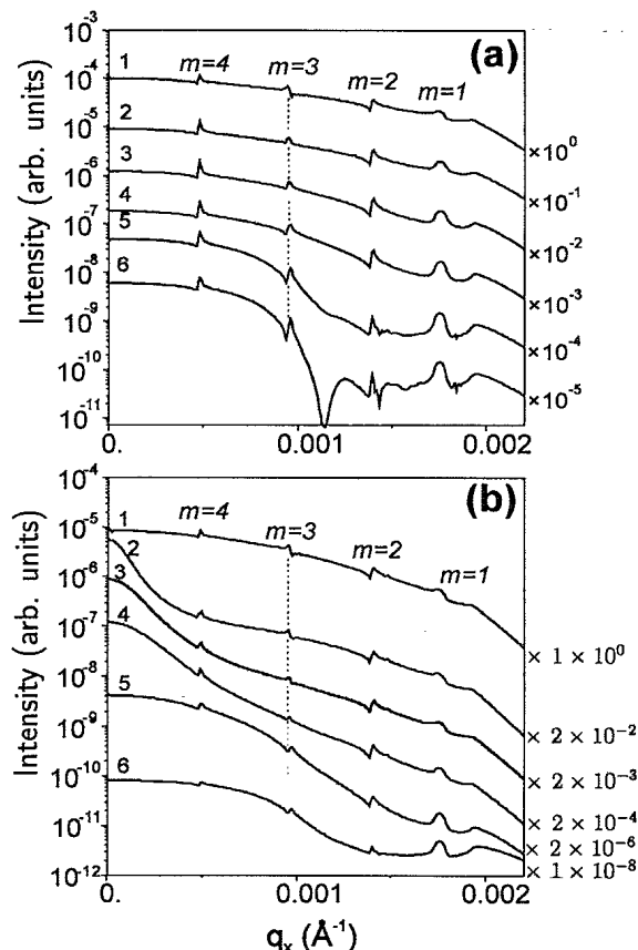
FIG. 2. Transformation of Bragg peaks in the section q_x = \text{const} along the fifth resonance sheet with an increase in the vertical correlation length of interface roughness for models of nonaccumulated (a) and accumulated (b) roughness. Lines 1–6 correspond to \xi_{\text{vert}} = 0, 200, 500, 1000, 10\,000, and \infty Å, respectively. The vertical dotted line follows the transformation of the third-order Bragg peak. The parameters of calculations are the same as in Fig. 1 with the exception of acquired rms roughness in (b): \sigma_{n < N} = 1.6 Å and \sigma_N = 8.6 Å.
